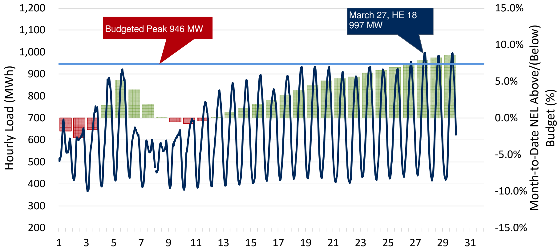
March 2020 Hourly ARP Loads (MWh) and Month to Date NEL vs. Budget (%)
