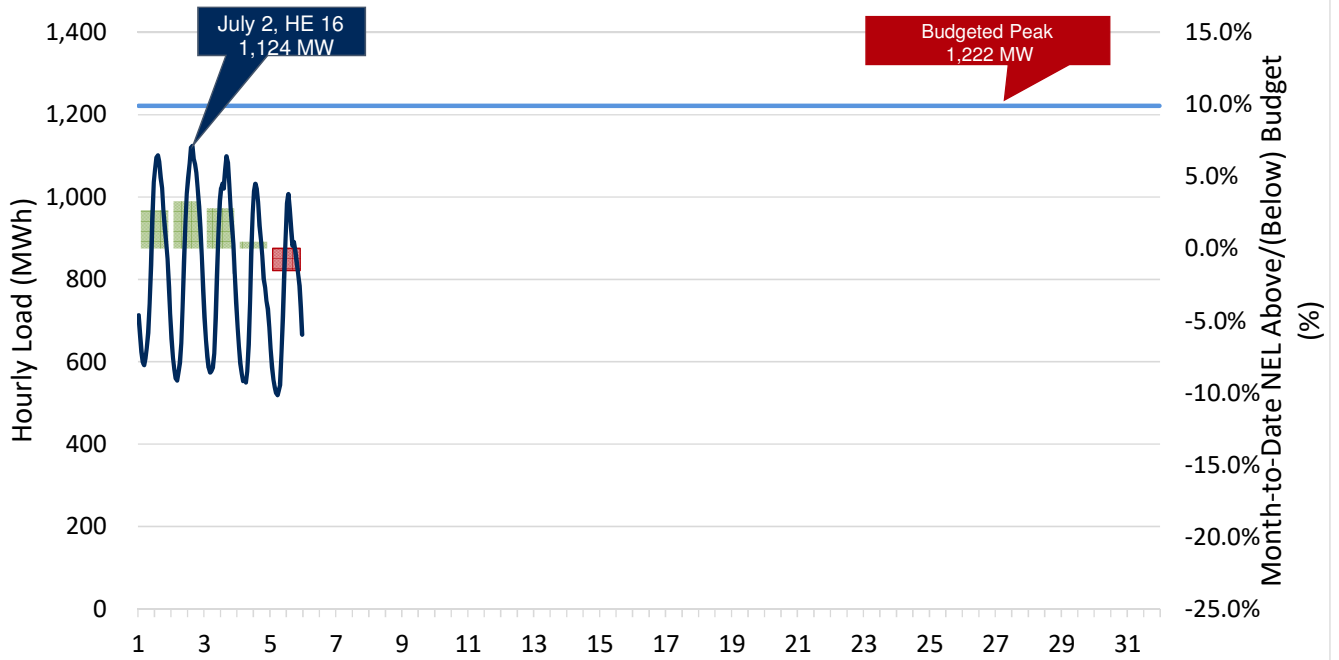
July 2020 Hourly ARP Loads (MWh) and Month to Date NEL vs. Budget (%)
