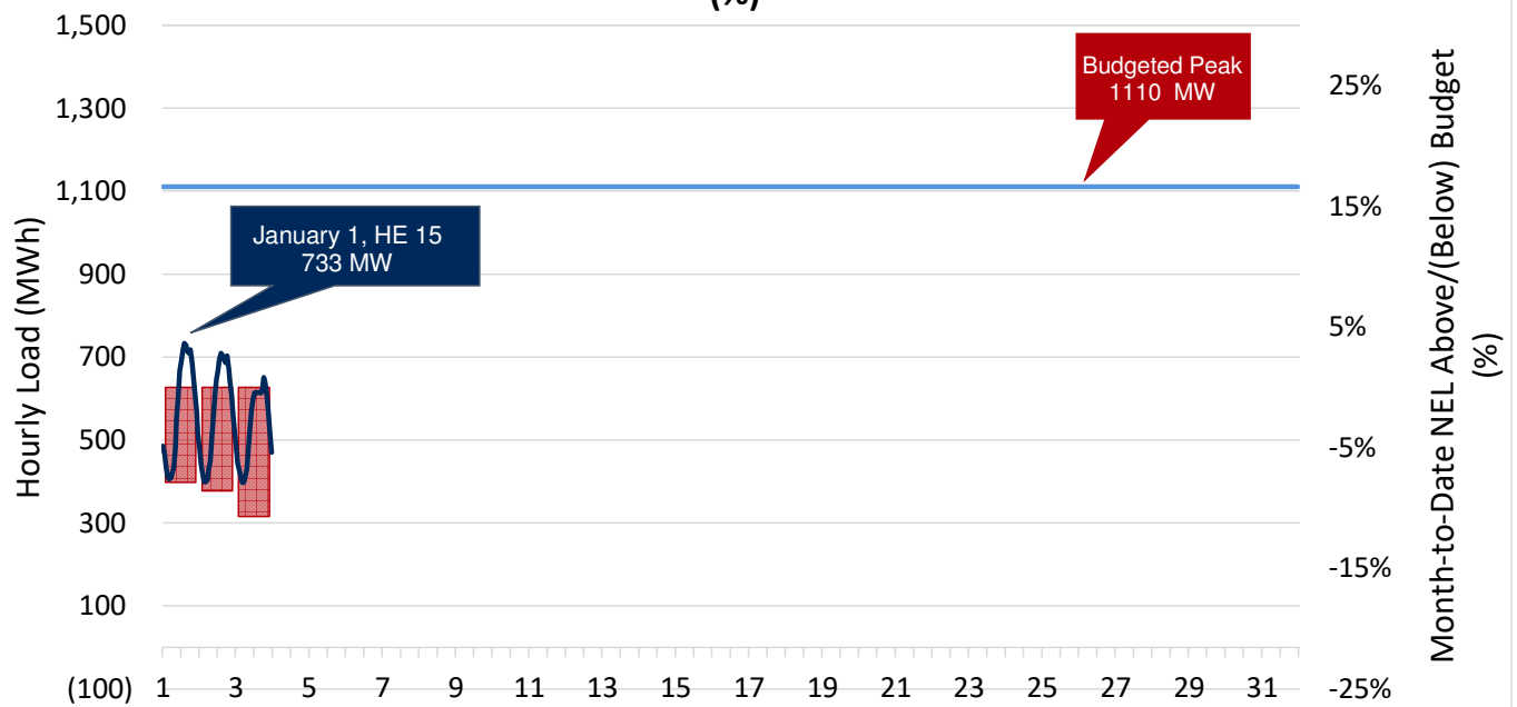
December 2020 Hourly ARP Loads (MWh) and Month to Date NEL vs. Budget (%)
