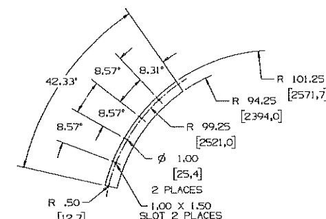
412 MAT'L: PLATE .38 THK A240-T321 SS
