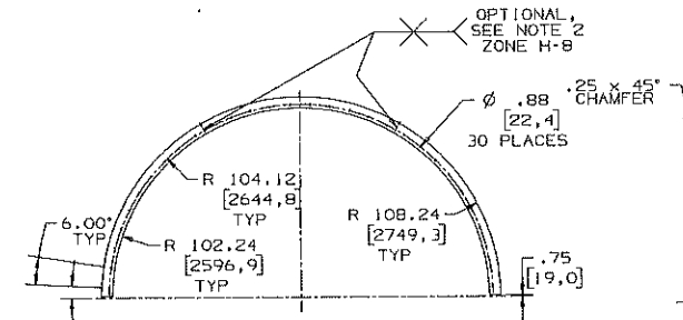
AFT FLANGE MAT'L: PLATE (104) .50 THK A36 CS
