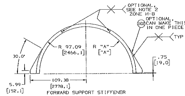
FORWARD SUPPORT STIFFENER
