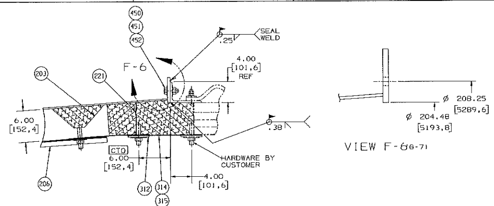
SECTION G-7 (C-3, SH.1) CUSTOMER SUPPLIED EXPANSION JOINT CTQ: SEE NOTE 22
