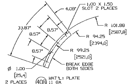
408 MAT'L: PLATE 11 GA A240-T321 SS
