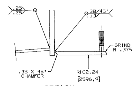
OPTION INTEGRATED EXP JOINT FLANGE OTHERWISE SAME AS SECTION D-7
