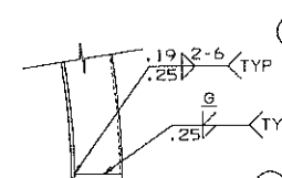
SECTION D-3 (D-5)
