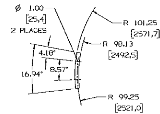
404 MAT'L: PLATE .19 THK A240-T321 SS
