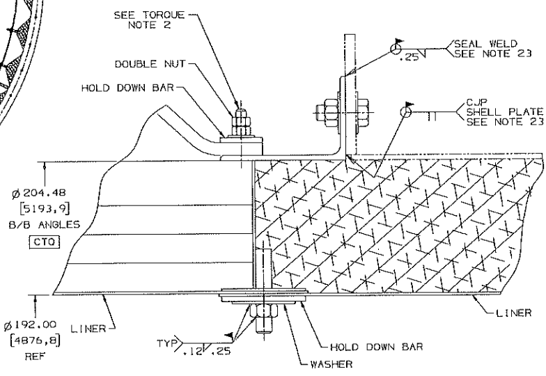
TYPICAL WELDING DETAIL E-2 STUDS & NUTS ON AFT EXPANSION JOINT
