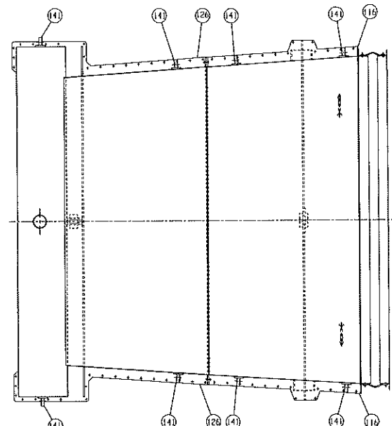
SECTION E-5 (D-5)
