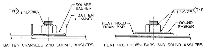
WELDING DETAIL - STUDS & NUTS
