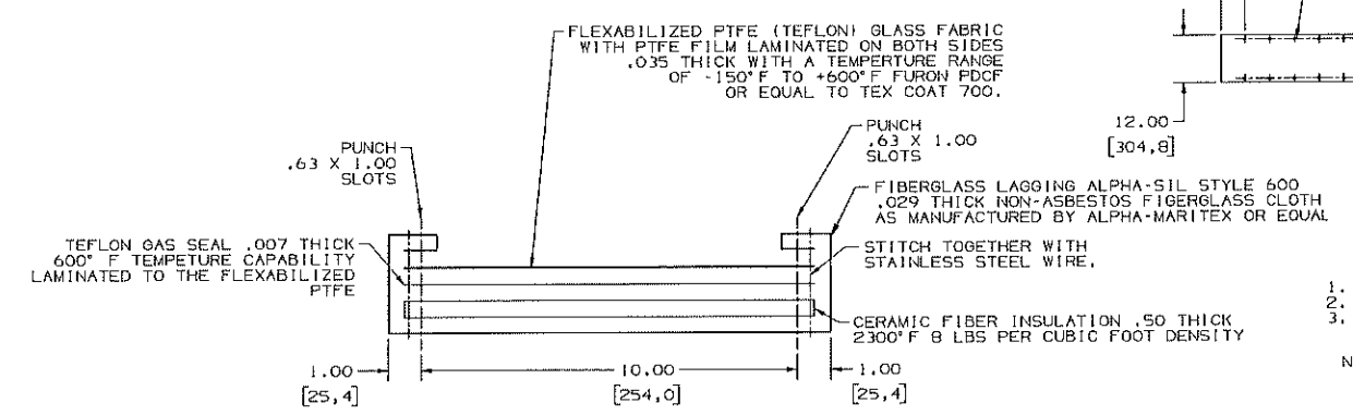
BELT MATERIAL DETAIL
