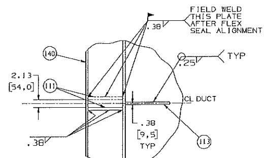
VIEW A-8
