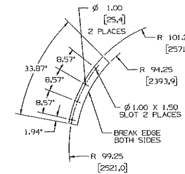
401 MAT'L: PLATE .38 THK A240-T321 SS
