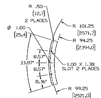
413 MAT'L: PLATE .38 THK A240-T321 SS
