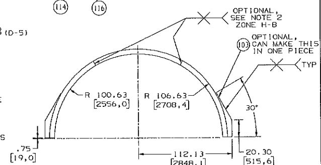
AFT SUPPORT UPPER STIFFENER
