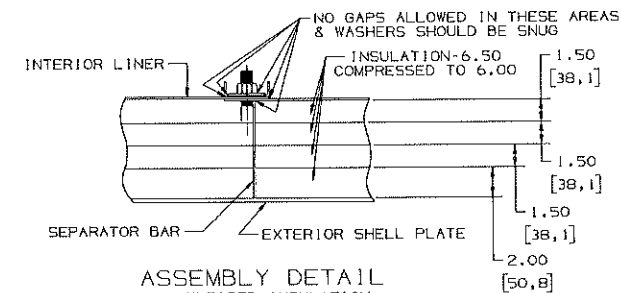
ASSEMBLY DETAIL NO EXPOSED INSULATION
