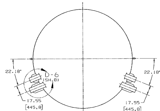
SECTION E-7(E-5) COMPRESSOR BLEED PIPING
