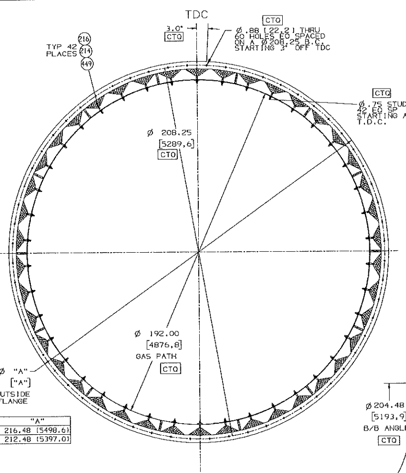
VIEW D-4 (D-3, SH.1)
