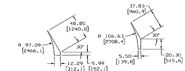
102 MAT'L: PLATE .75 THK. A36 CS
