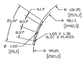
406 MAT'L: PLATE .19 THK A240-T321 SS
