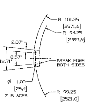
400 MAT'L: PLATE .38 THK A240-T321 SS
