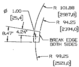
409 MAT'L: PLATE 11 GA A240-T321 SS
