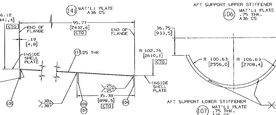
AFT SUPPORT UPPER STIFFENER
