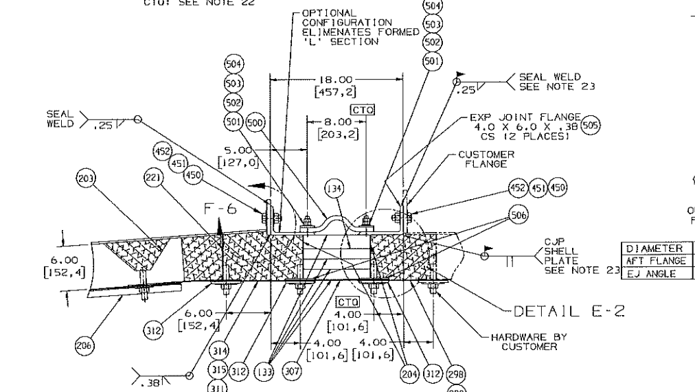
SECTION D-7 (C-3, SH.1) G.E. SUPPLIED EXPANSION JOINT CTQ: SEE NOTE 22
