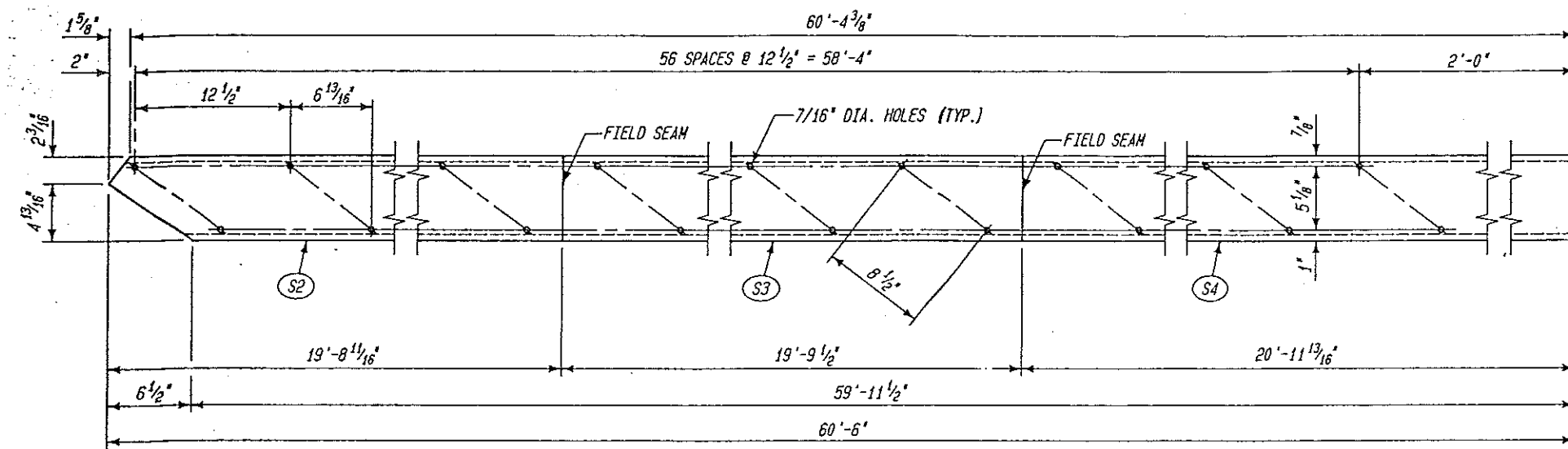
DETAIL OF INNER STRINGER - ITEMS "S2", "S3", & "S4" FLIP OVER TO ROLL
