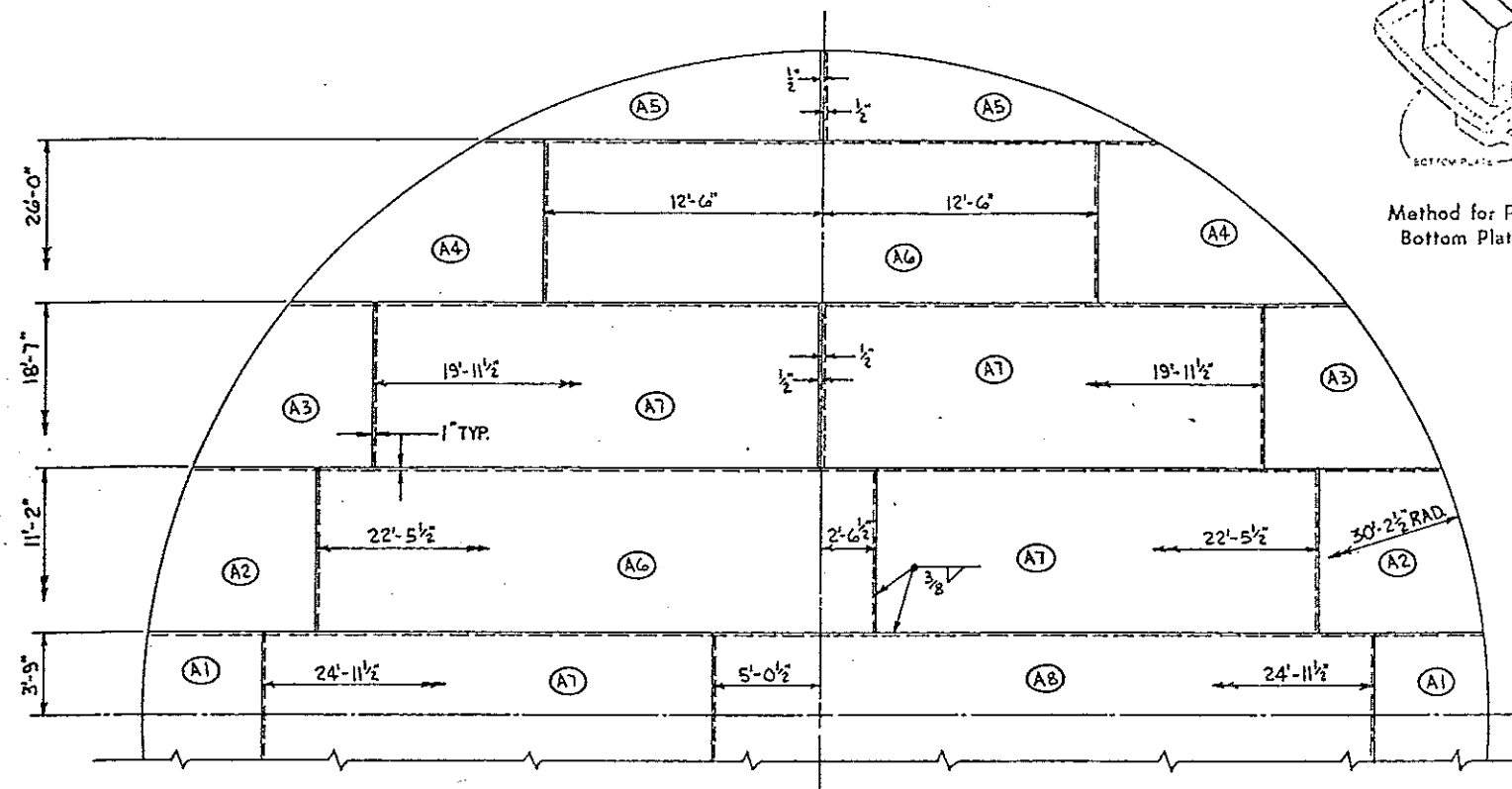
PARTIAL PLAN VIEW OF BOTTOM
