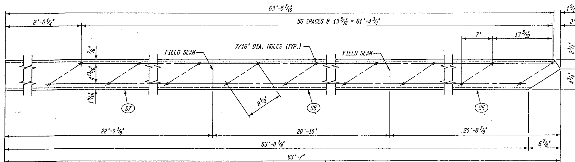
DETAIL OF OUTER STRINGER - ITEMS "S5", "S6", & "S7" ROLL THIS SIDE UP AS SHOWN
