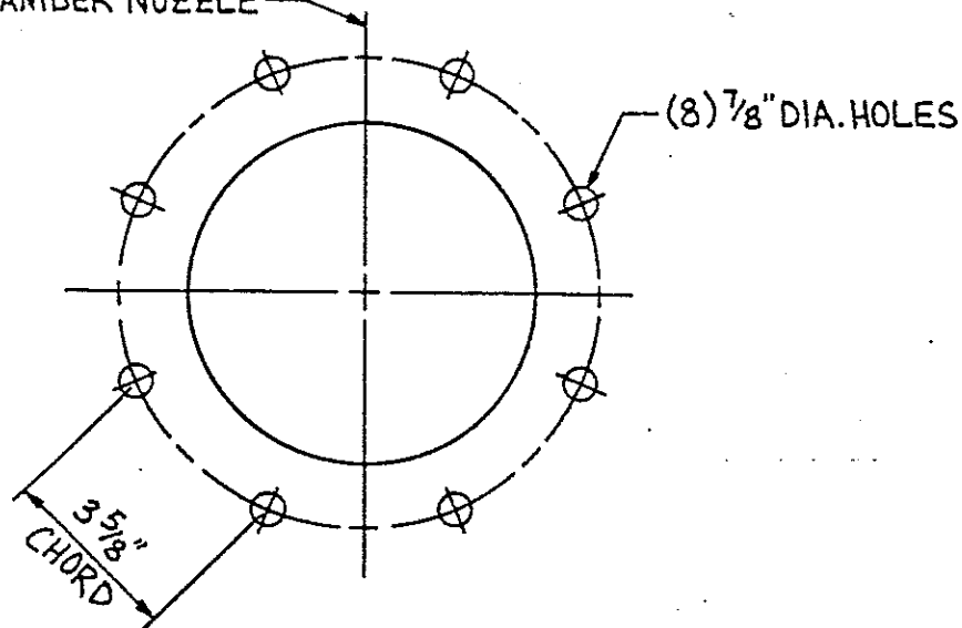
VIEW "A-A"
